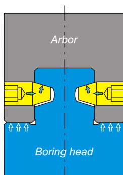
➤ Tapered screws
