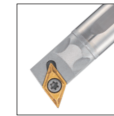
SDUC□95°
