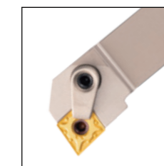
MCLN□95°
