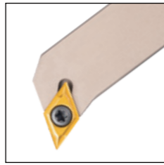
SDQC□107.5°
