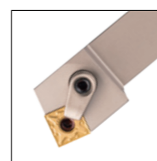
MSRN□75°
